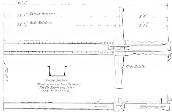
Half Section of the Underframe Used by the Marsh Refrigerator Service Company
